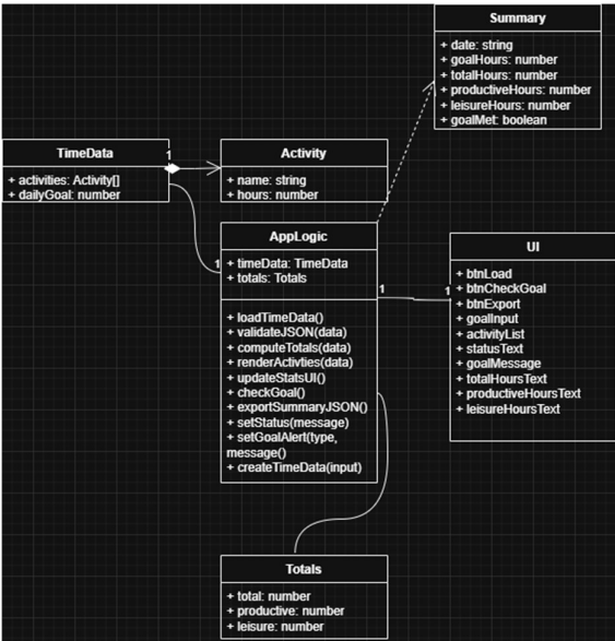
Figure 3 Class Diagram, system structure including data, logic and UI layers
