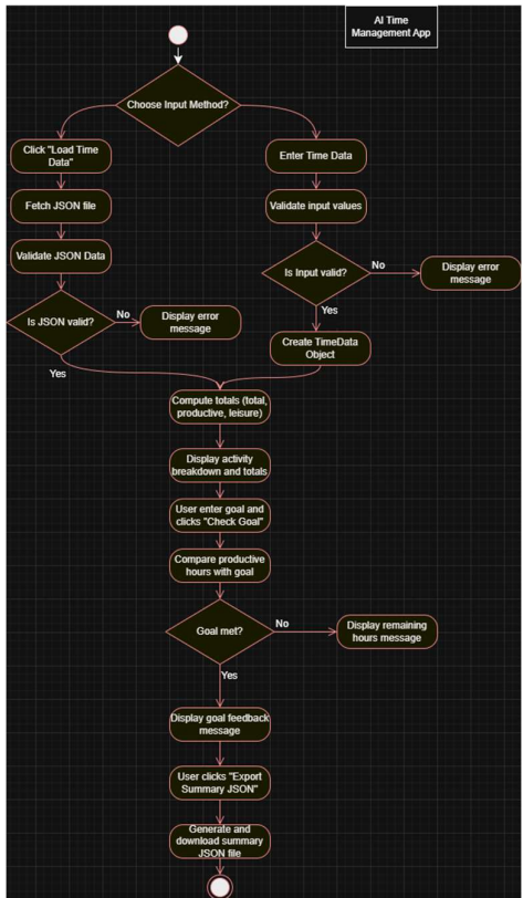
Figure 1 Activity Diagram, showing data input, processing and feedback
