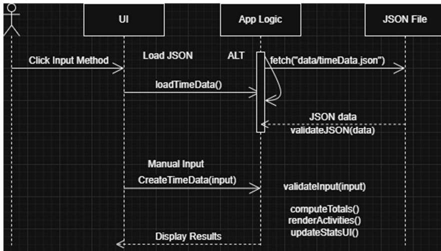
Figure 4 Sequence Diagram
