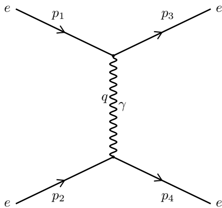
t -channel, q = p_1 - p_3
