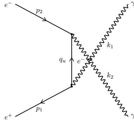
u-channel, q_u = p_2 - k_2
