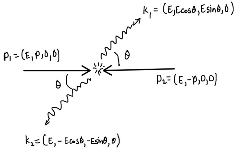
Figure 7: Pair Annihilation in COM
