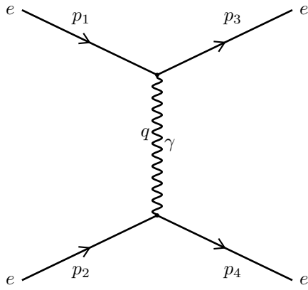
t -channel, q = p_1 - p_3
