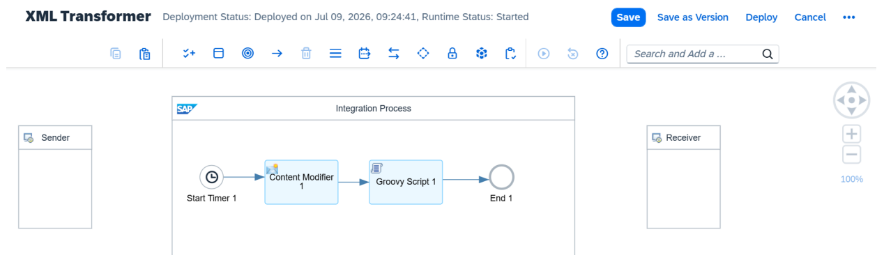
Figure 1: Timer -> Content Modifier -> Groovy Script -> End
