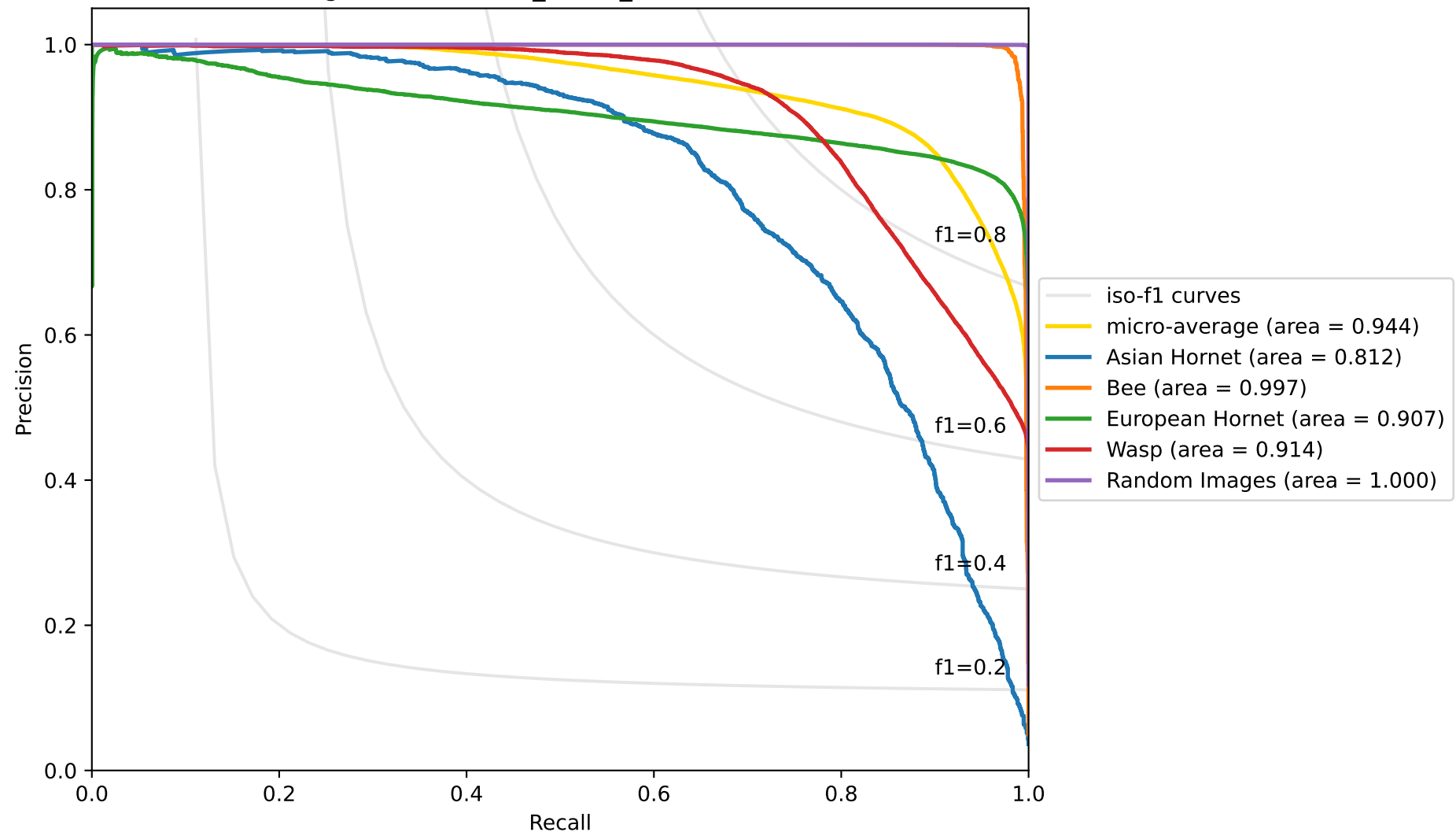
Average Precision / PR_Curve_AUC micro: 0.9445
