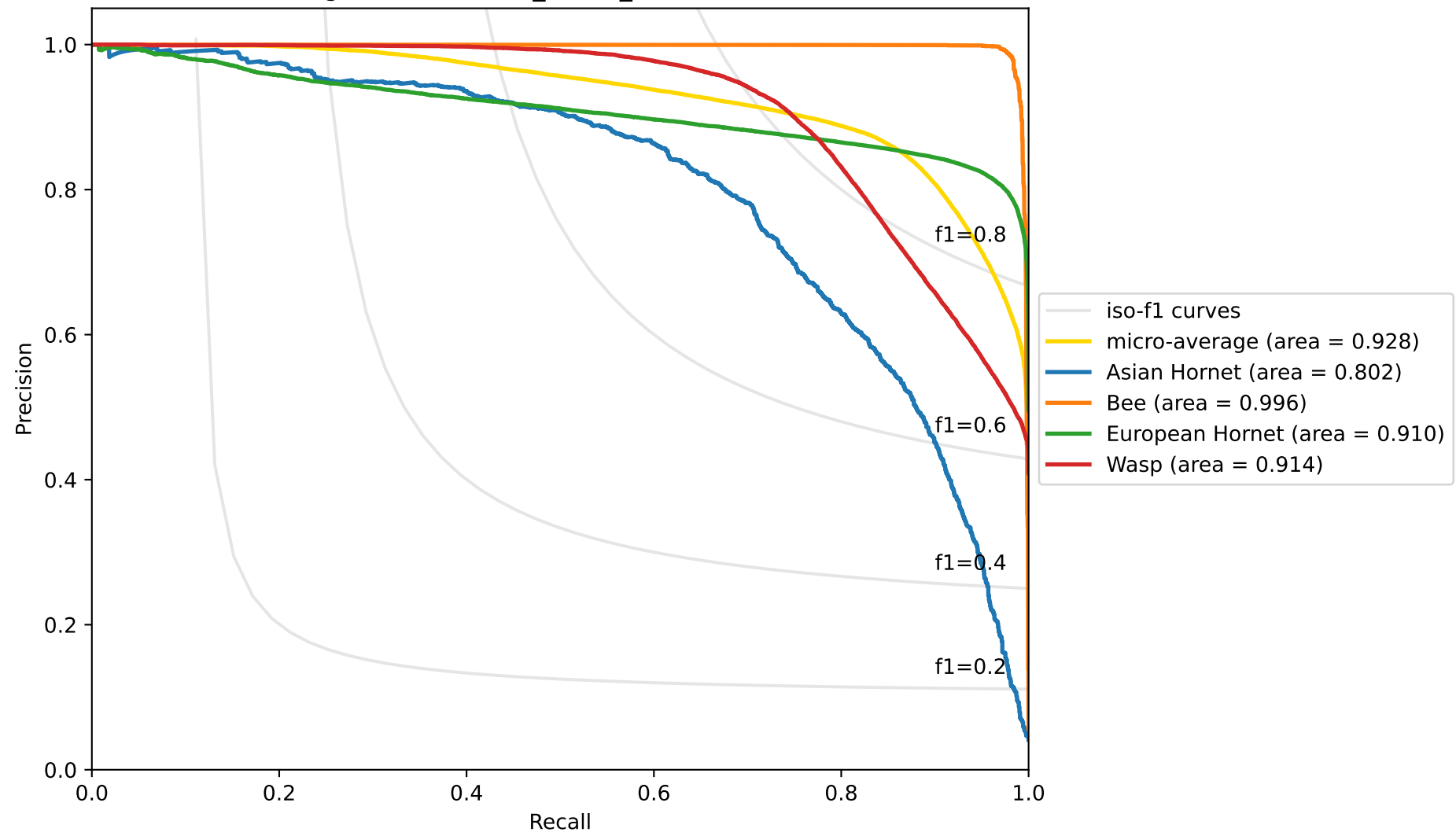
Average Precision / PR_Curve_AUC micro: 0.9276
