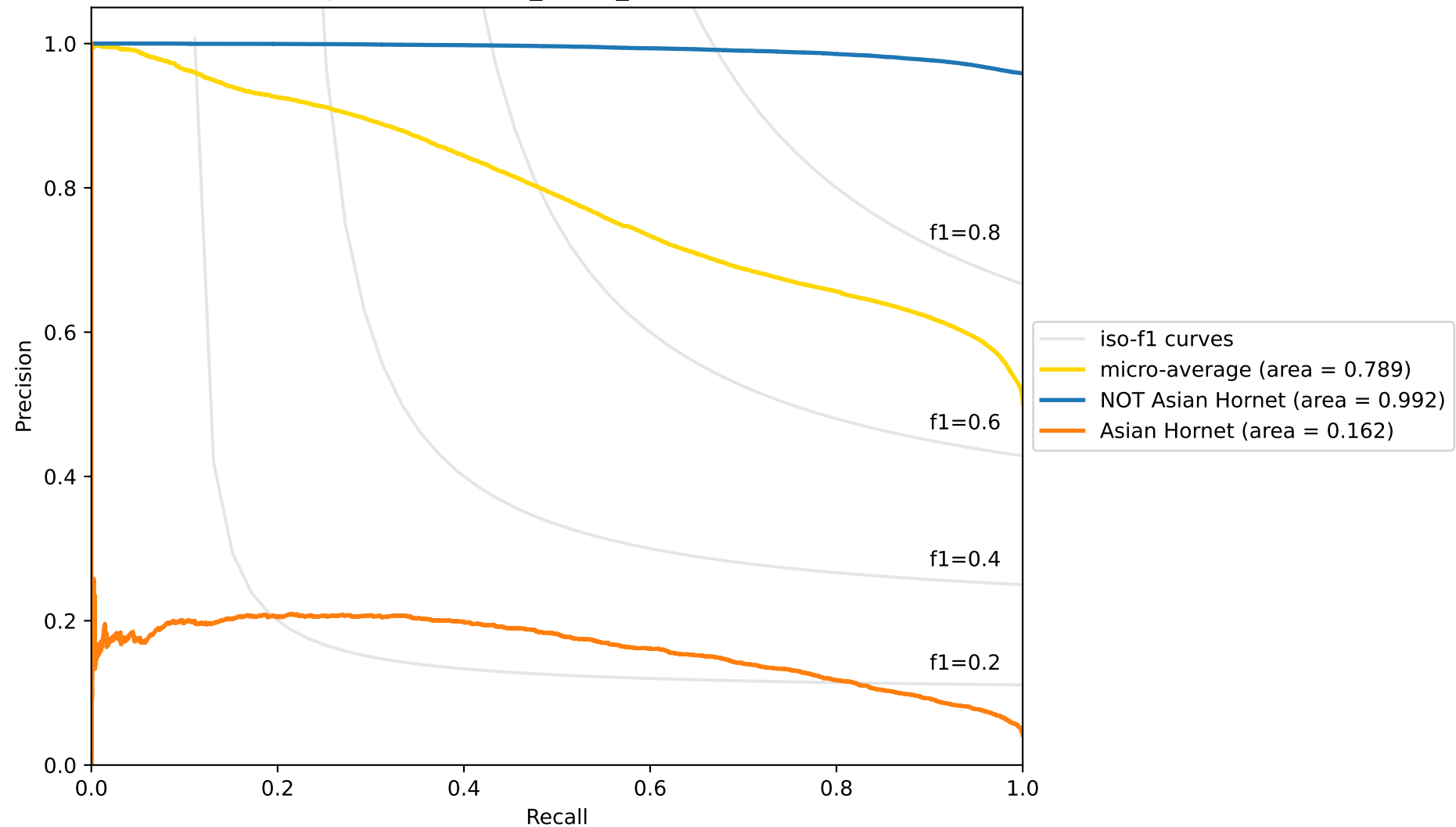
Average Precision / PR_Curve_AUC micro: 0.7892
