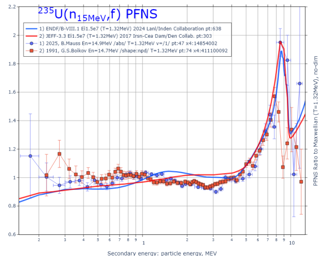
FIG. 12. Ratio of measured PFNS by a 1.32 MeV Maxwellian distribution for four incoming neutron energies. The horizontal bars give the bin size while the points are placed at the mean energy position of the energy distribution within each bin. The JEFF3.3 and ENDF/B VIII.1 evaluations are plotted for comparison. Data from Refs. [4,29,30] were also added for comparison. The corresponding energies are given in the legend.
