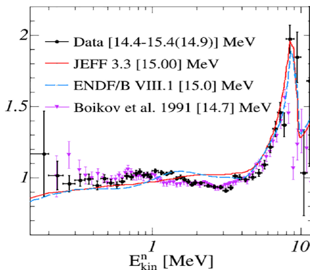
FIG. 12. Ratio of measured PFNS by a 1.32 MeV Maxwellian distribution for four incoming neutron energies. The horizontal bars give the bin size while the points are placed at the mean energy position of the energy distribution within each bin. The JEFF3.3 and ENDF/B VIII.1 evaluations are plotted for comparison. Data from Refs. [4,29,30] were also added for comparison. The corresponding energies are given in the legend.
