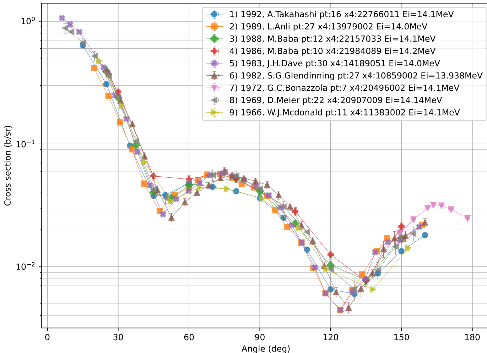
Plot EXFOR angular distributions d\sigma/d\Omega(E,\theta) : O-16(n,el),da X4Pro, by V.Zerkin, IAEA-NDS, 2021-2022, ver.2022-12-20 //running:2026-08-25 23:09:45
