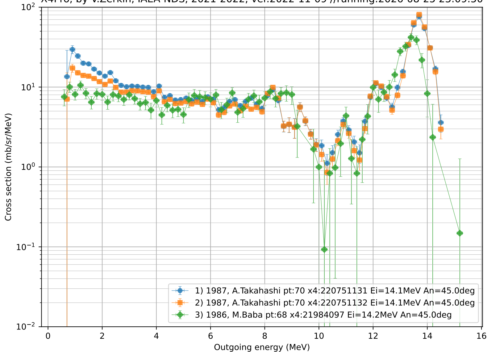
Plot EXFOR double differential cross sections: F-19(n,xn),dae X4Pro, by V.Zerkin, IAEA-NDS, 2021-2022, ver.2022-11-09 //running:2026-08-25 23:09:50
