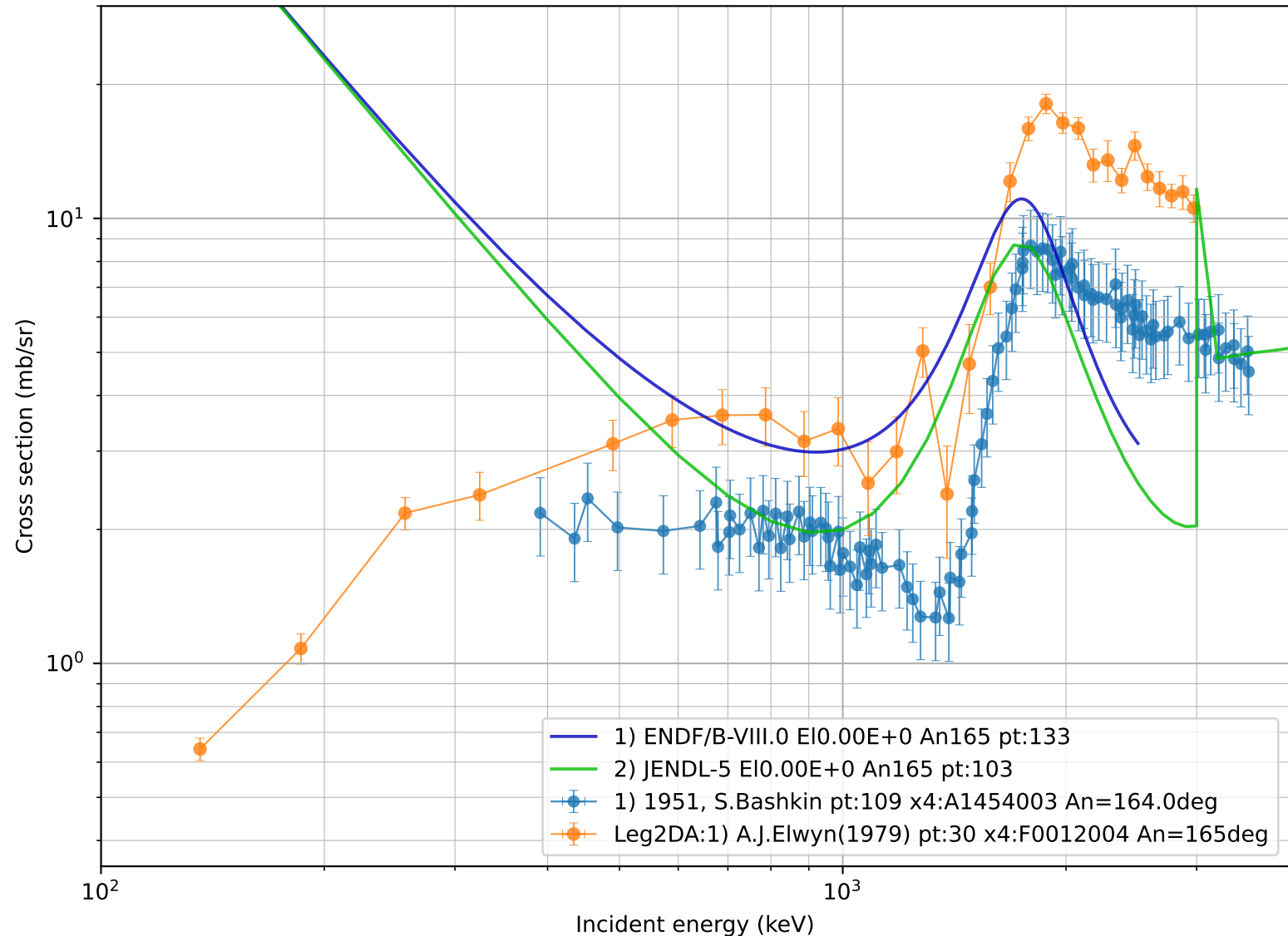
Plot EXFOR/ENDF angular distributions d\sigma/d\Omega(E,\theta) : Li-6(p,he3),da X4Pro, by V.Zerkin, IAEA-NDS, 2021-2022, ver.2022-12-07 //running:2026-08-25:23:11:05
