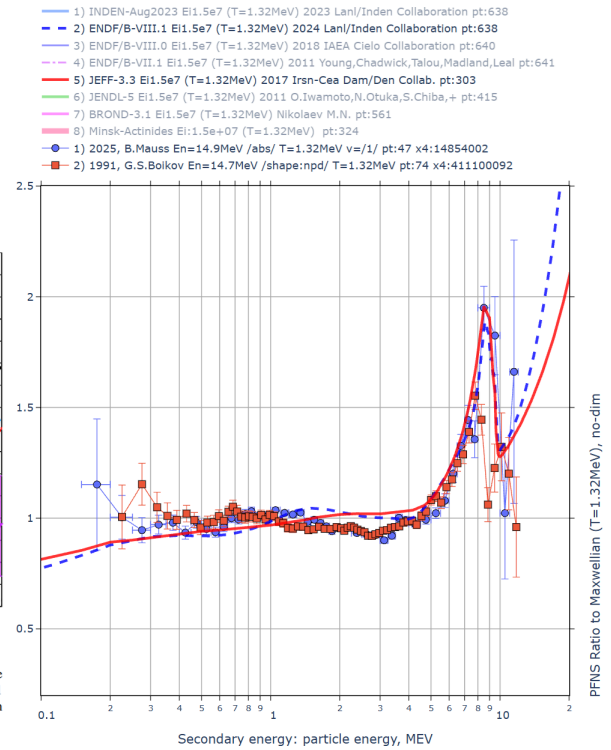
FIG. 12. Ratio of measured PFNS by a 1.32 MeV Maxwellian distribution for four incoming neutron energies. The horizontal bars give the bin size while the points are placed at the mean energy position of the energy distribution within each bin. The JEFF3.3 and ENDF/B VIII.1 evaluations are plotted for comparison. Data from Refs. [4,29,30] were also added for comparison. The corresponding energies are given in the legend.
