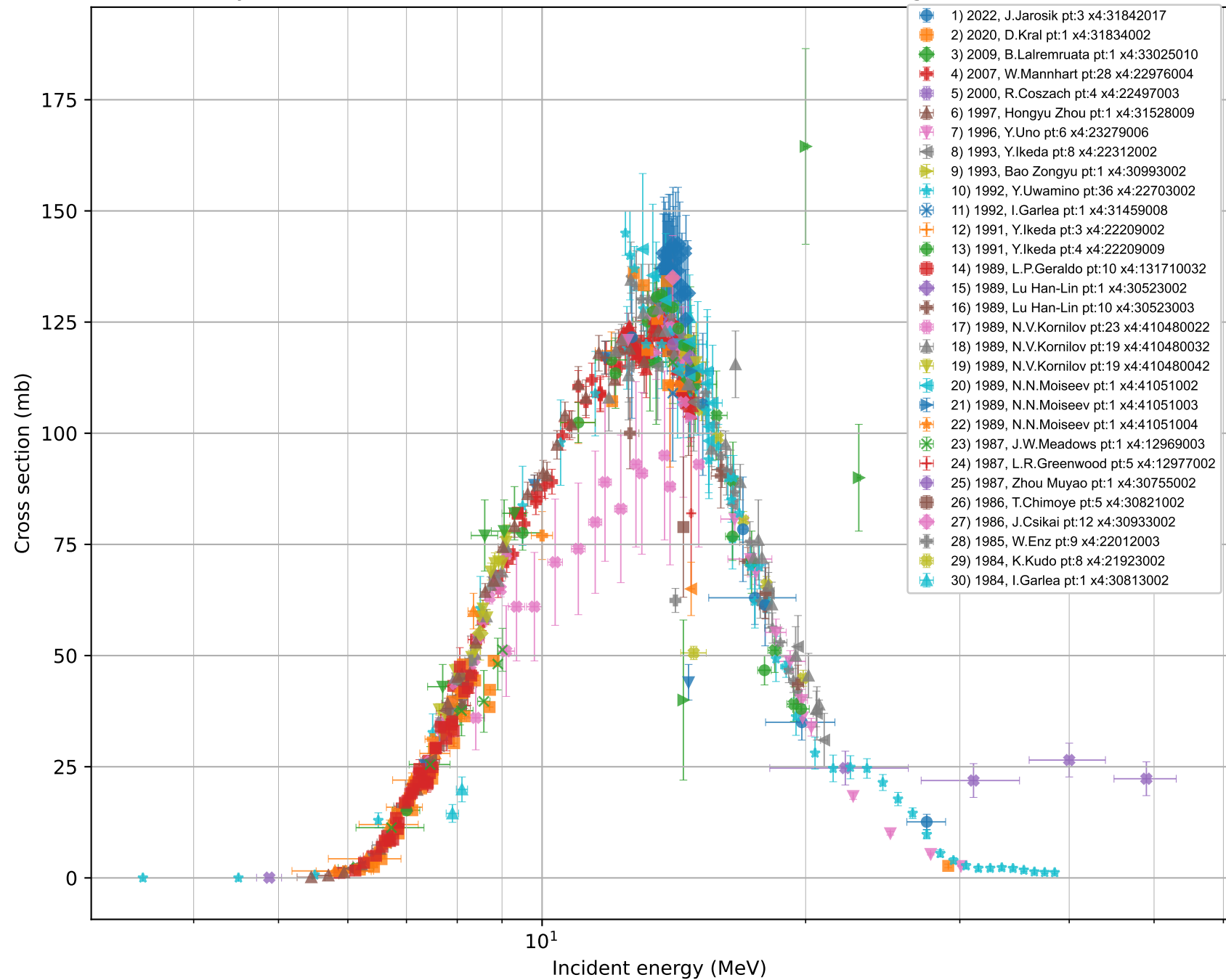
EXFOR cross sections \sigma(E) : Al-27(n,a),sig X4Pro, by V.Zerkin, IAEA-NDS, 2021-2022, ver.2022-11-09 //running:2026-08-12 14:33:20
