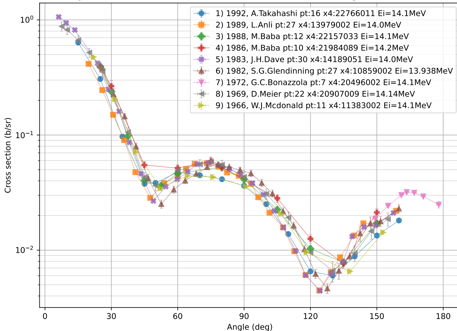
Plot EXFOR angular distributions d\sigma/d\Omega(E,\theta) : O-16(n,el),da X4Pro, by V.Zerkin, IAEA-NDS, 2021-2022, ver.2022-12-20 //running:2026-08-12 14:33:23
