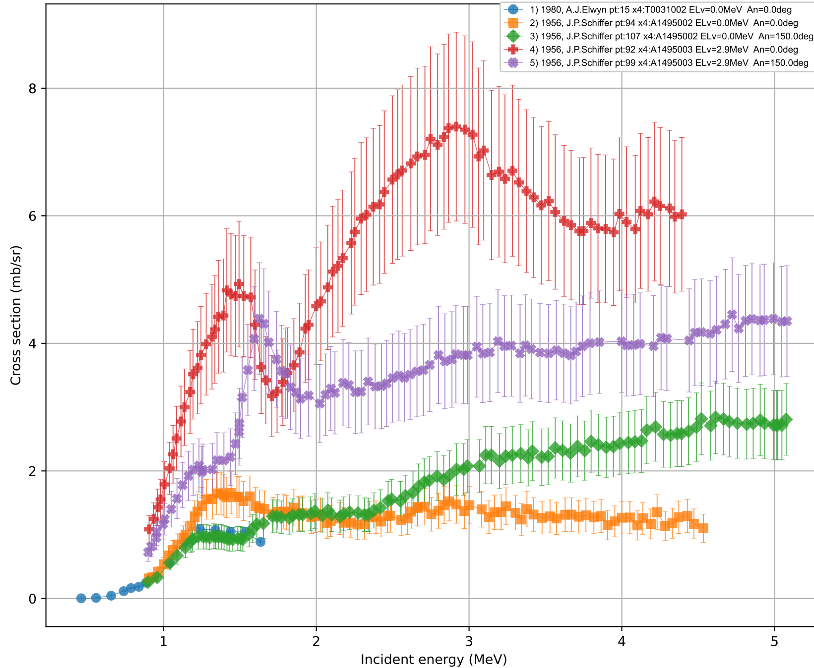
Plot EXFOR angular distributions d\sigma/d\Omega(E,\theta) : Li-6(he3,p)par,da X4Pro, by V.Zerkin, IAEA-NDS, 2021-2022, ver.2022-11-09 //running:2026-08-12 14:33:25
