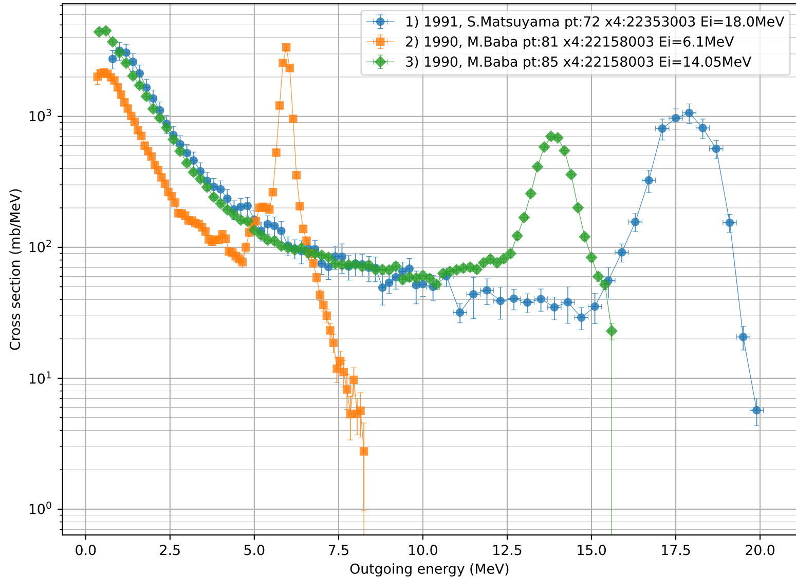
Plot EXFOR emission spectra d\sigma/dE_{out} : Th-232(n,xn),de X4Pro, by V.Zerkin, IAEA-NDS, 2021-2022, ver.2022-12-20 //running:2026-08-12 14:33:26
