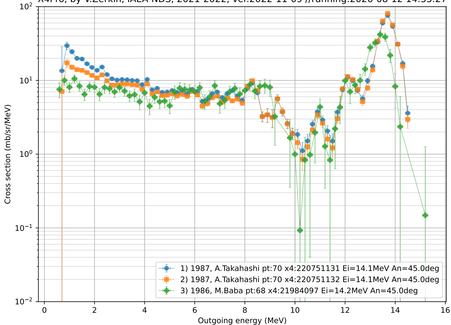
Plot EXFOR double differential cross sections: F-19(n,xn),dae X4Pro, by V.Zerkin, IAEA-NDS, 2021-2022, ver.2022-11-09 //running:2026-08-12 14:33:27
