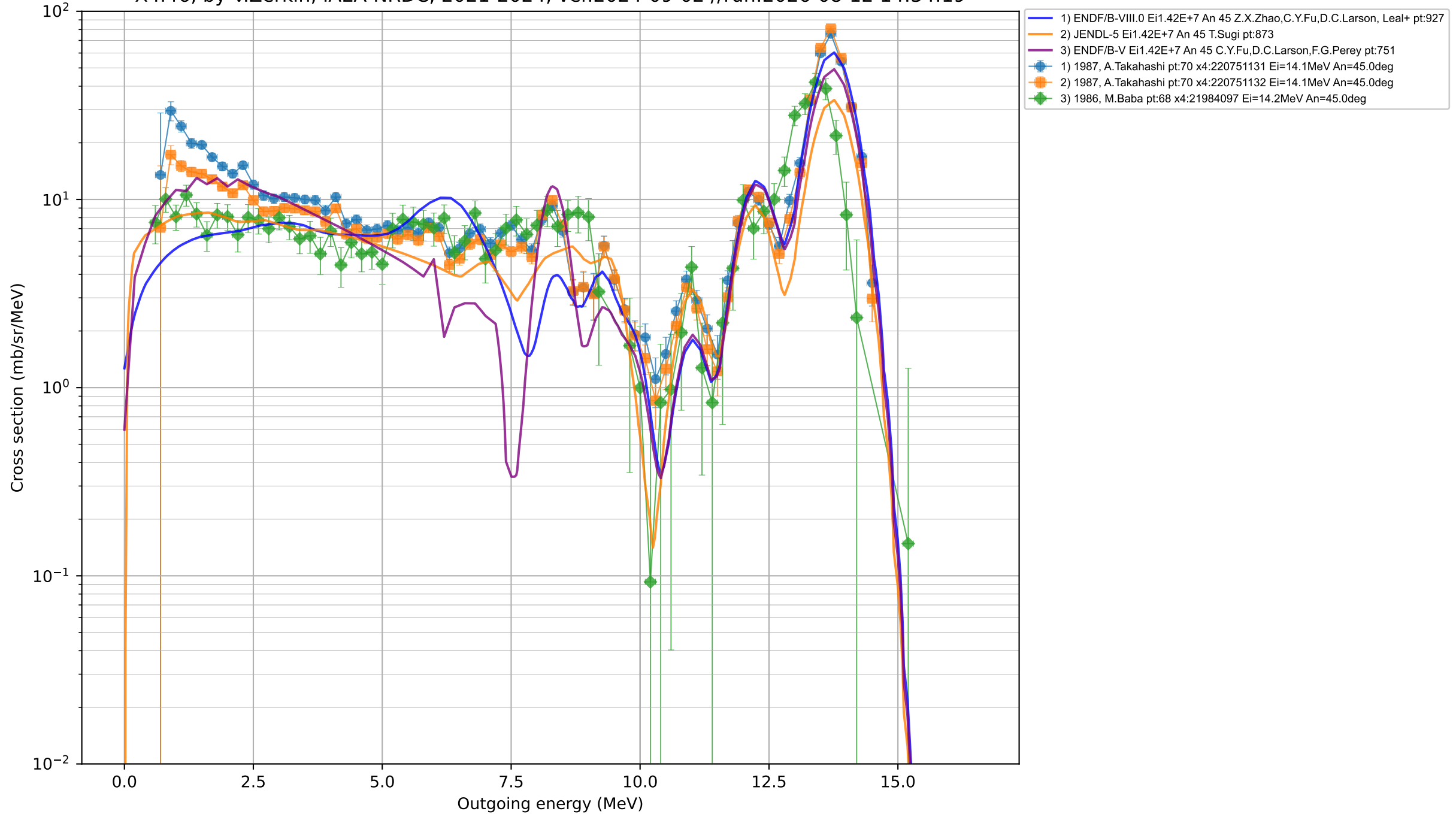
EXFOR/ENDF double differential cross sections: F-19(n,xn),dae X4Pro, by V.Zerkin, IAEA-NRDC, 2021-2024, ver.2024-09-02 //run:2026-08-12 14:34:19
