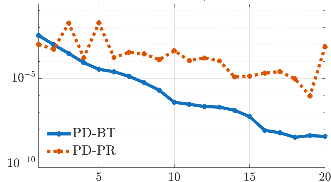
Adv-Diff Ratio c/a = 100
