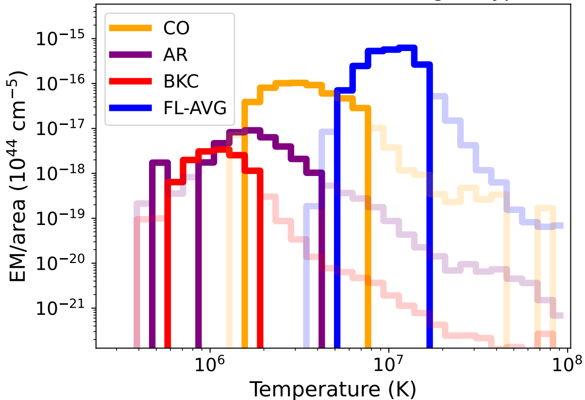
Restricted EMDs of coronal region types
