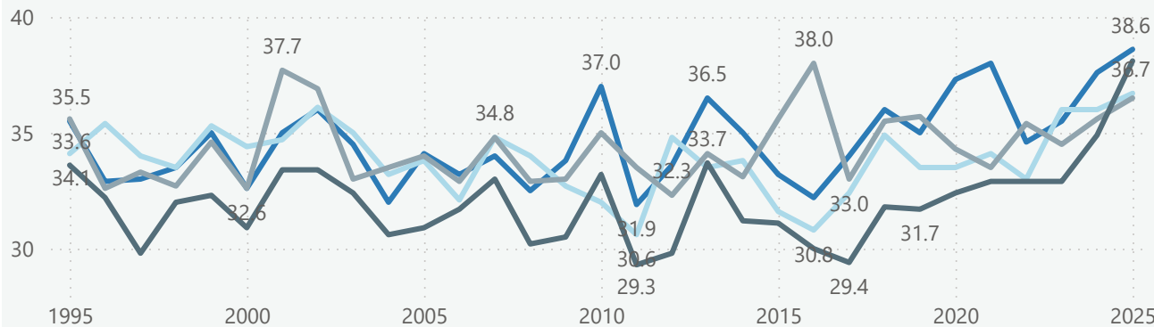
Correlation
