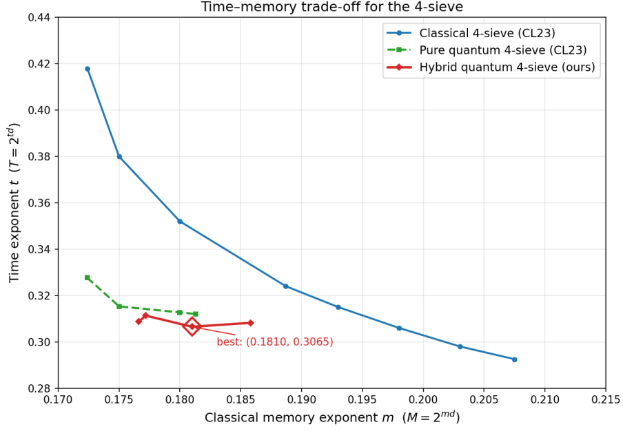
Figure 1: Time–memory trade-off for the 4-sieve.
