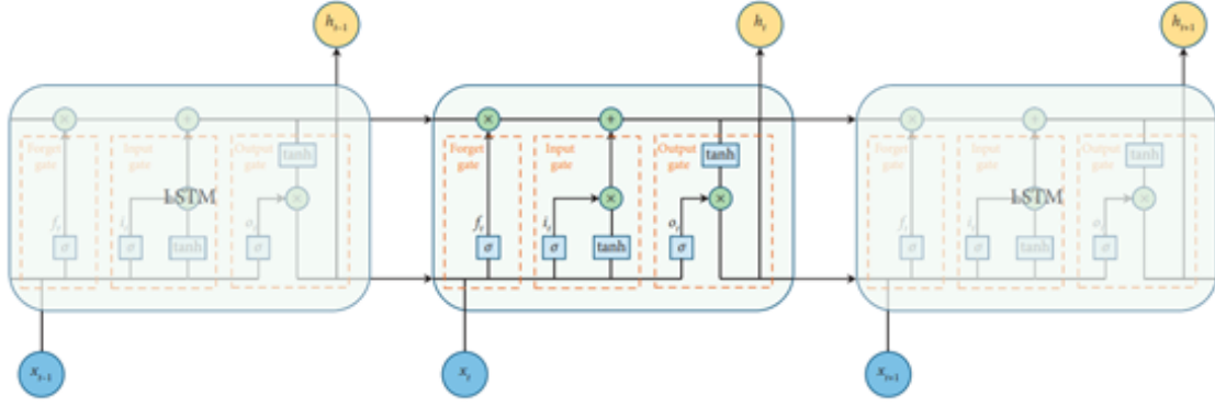
Figure 2.10 LSTM ARCHITECTURE
