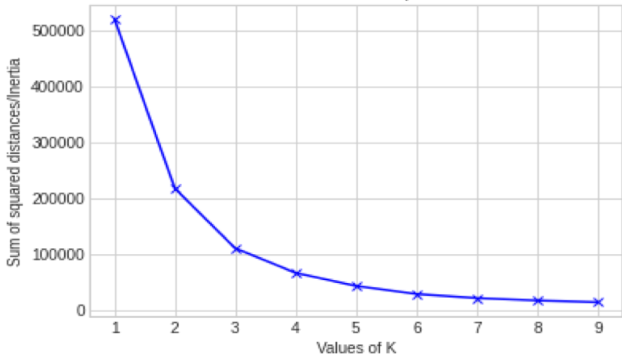
Figure 2.19 K-Means Clustering [6]
