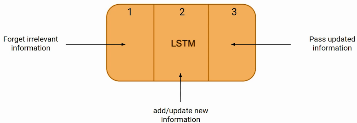
Figure 2.9 LSTM Cell
