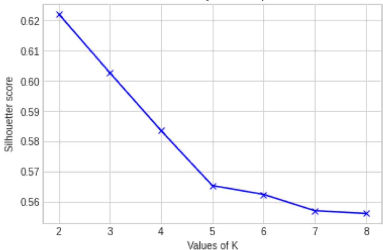
Figure 2.20 SILHOUETTE METHOD [6]
