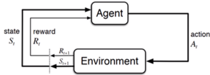
Figure 2.18 REINFORCEMENT LEARNING
