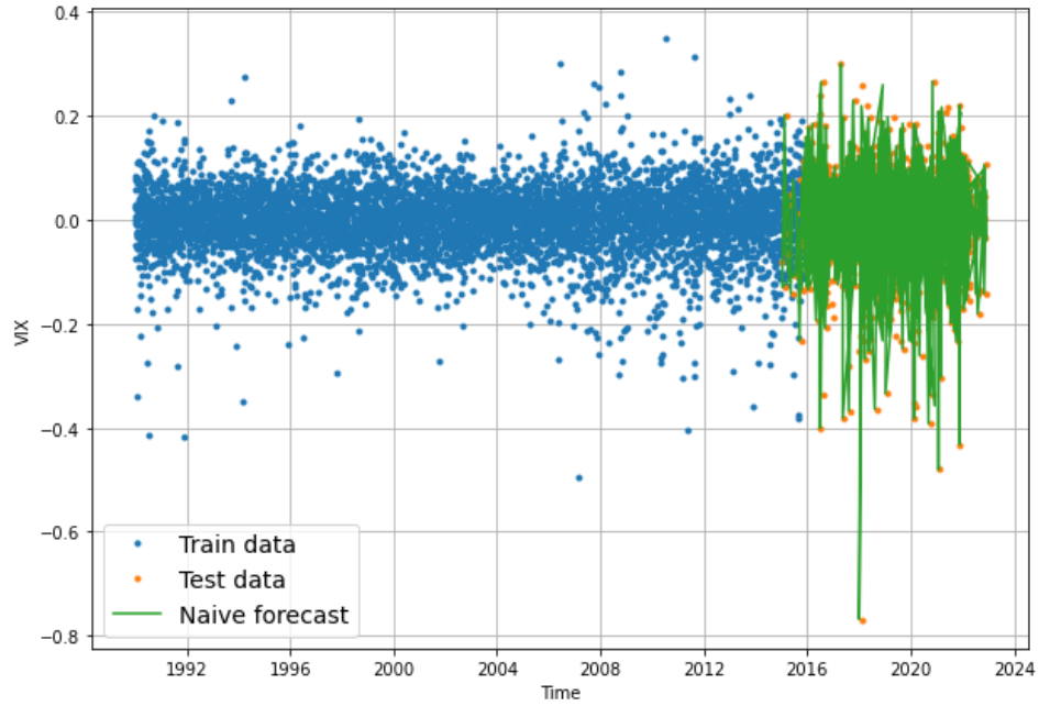
Figure 2.28 Naïve forecast [9]
