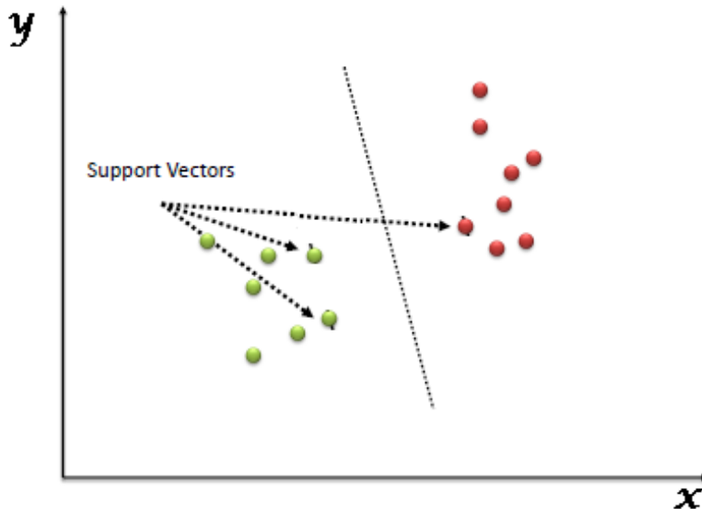
Figure 2.14 Hyperplane with Support Vectors
