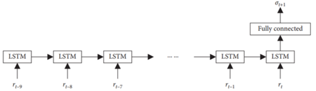
Figure 2.11 LSTM with Fully Connected Layer
