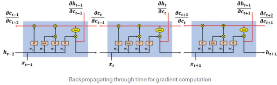
Figure 3.4: Source: [23] Gradient vanishing in LSTM.
