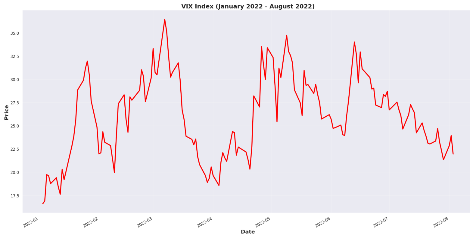
Figure 3.8: Time Series: VIX Hurst = 0.398, Lag 1, Lag 2 = 2, 20, Time: 03/01/2022 — 4/8/2022.
