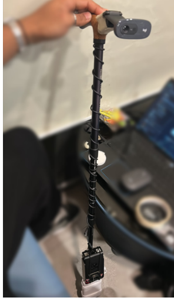
Figure 2: Assembled prototype: Raspberry Pi 4, Arducam ToF camera (CSI), and USB webcam.
