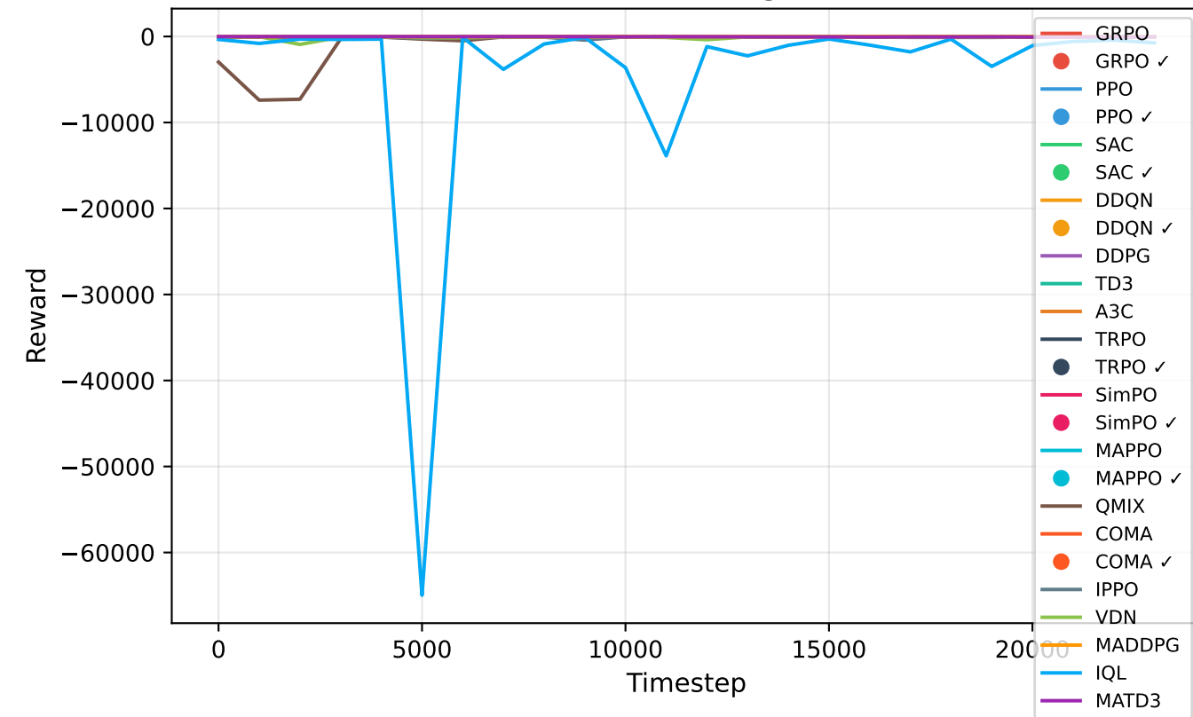
Reward Convergence
