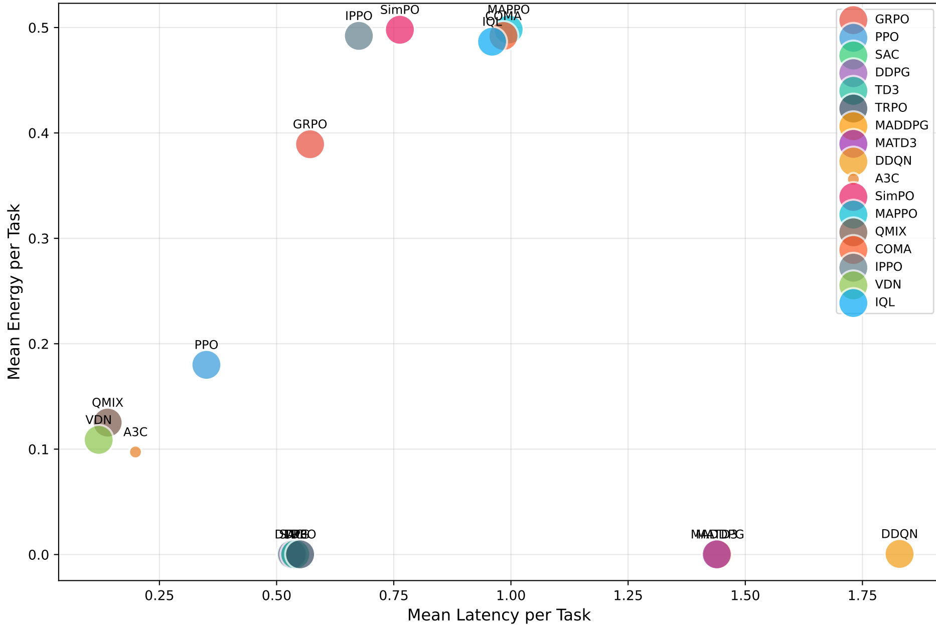
Latency vs Energy per Task (bubble size \propto |\text{reward}| )
