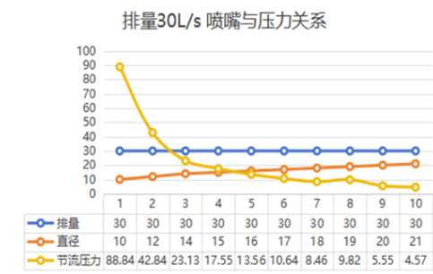
(c) 30L/s
