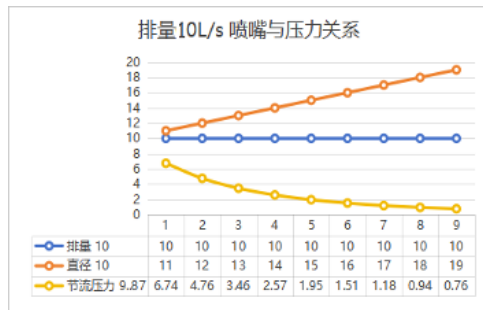
(a) 10L/s
