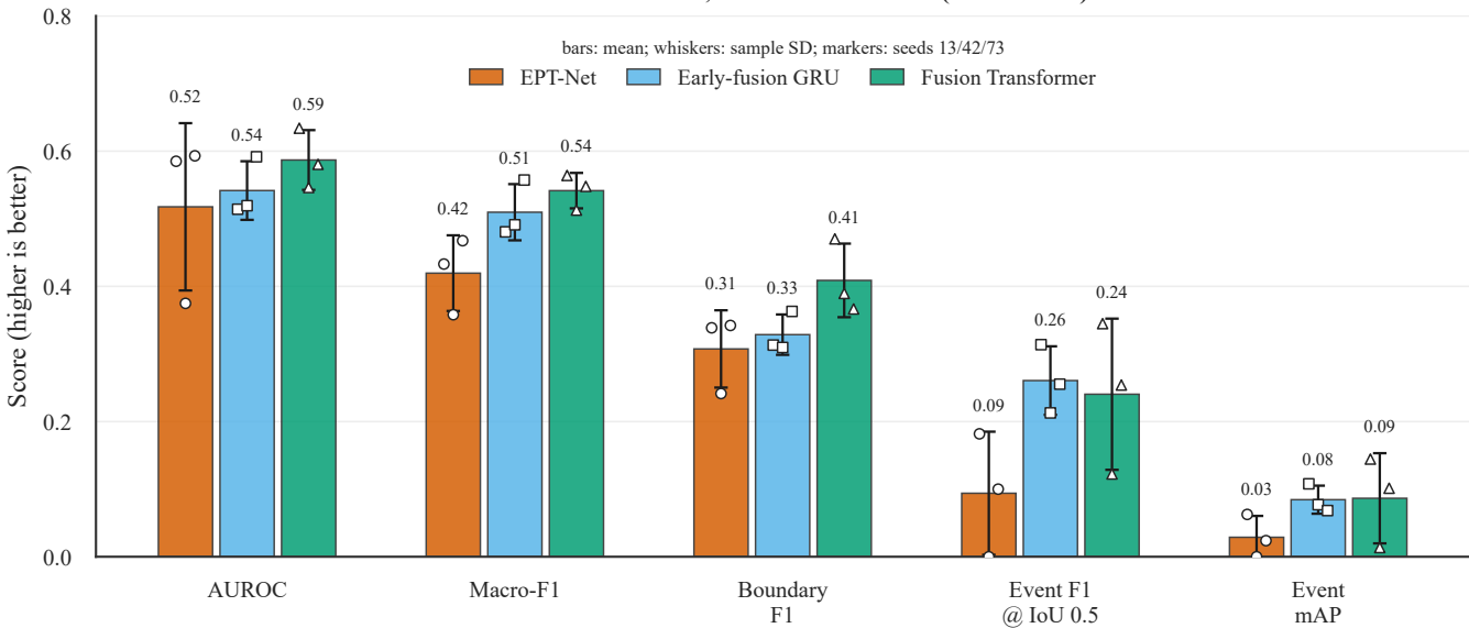
Continuous-session, no-text evaluation (three seeds)
