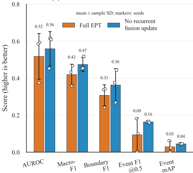
(a) Persistent-state ablation: 3 seeds
