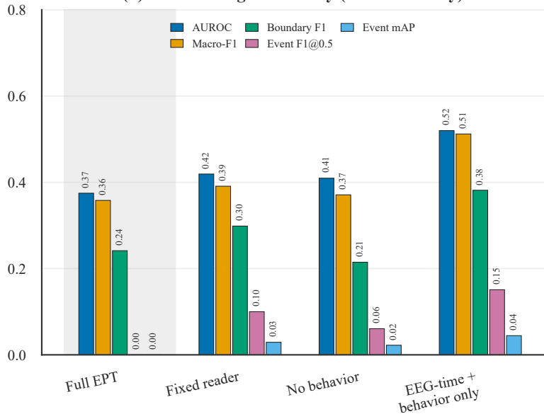
(b) Seed-42 diagnostics only (no uncertainty)
