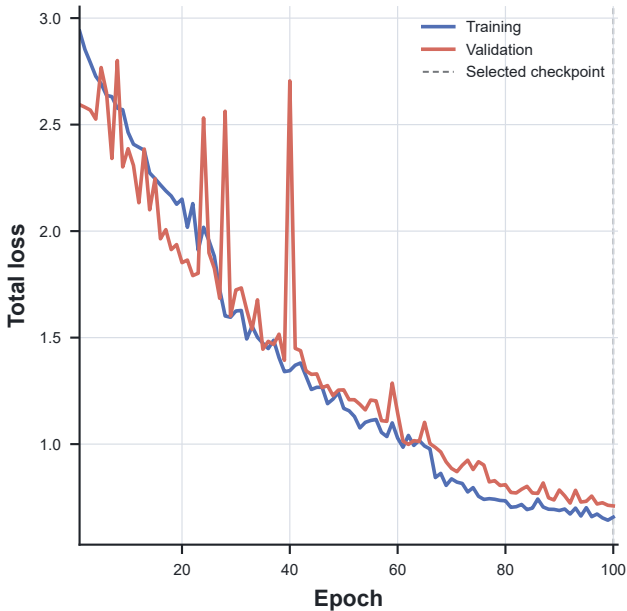
EPT-Net loss convergence
