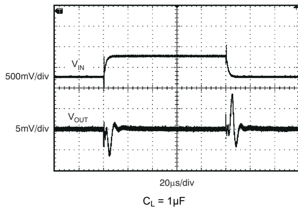
Figure 6-21. Line Transient
