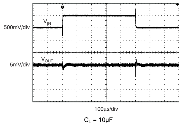
Figure 6-22. Line Transient
