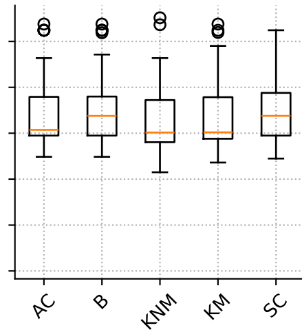
Completeness
