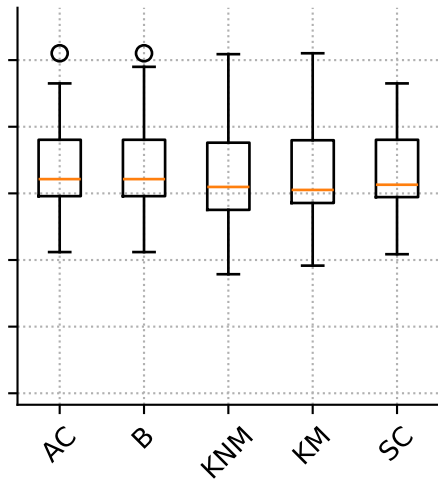
Homogeneity
