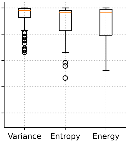
Homogeneity
