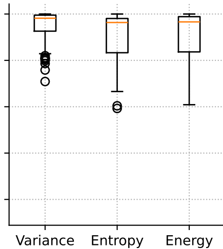
Completeness
