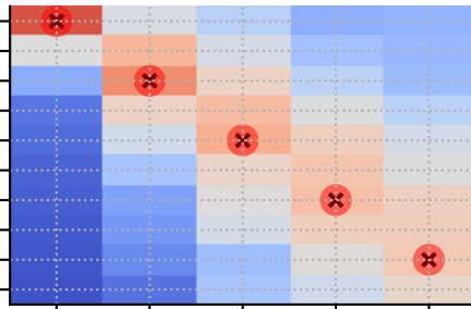
chunk size: 200
