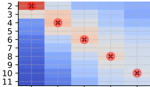
chunk size: 100
