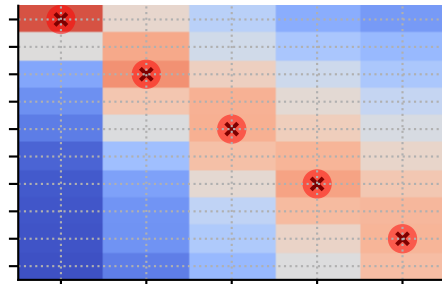
chunk size: 400
