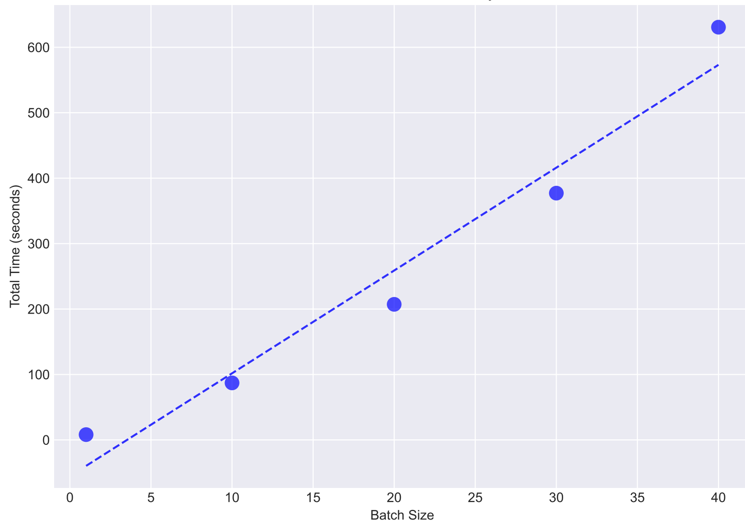
zkSNARK Time Scalability
