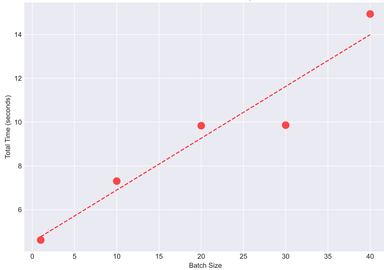
zkSTARK Time Scalability
