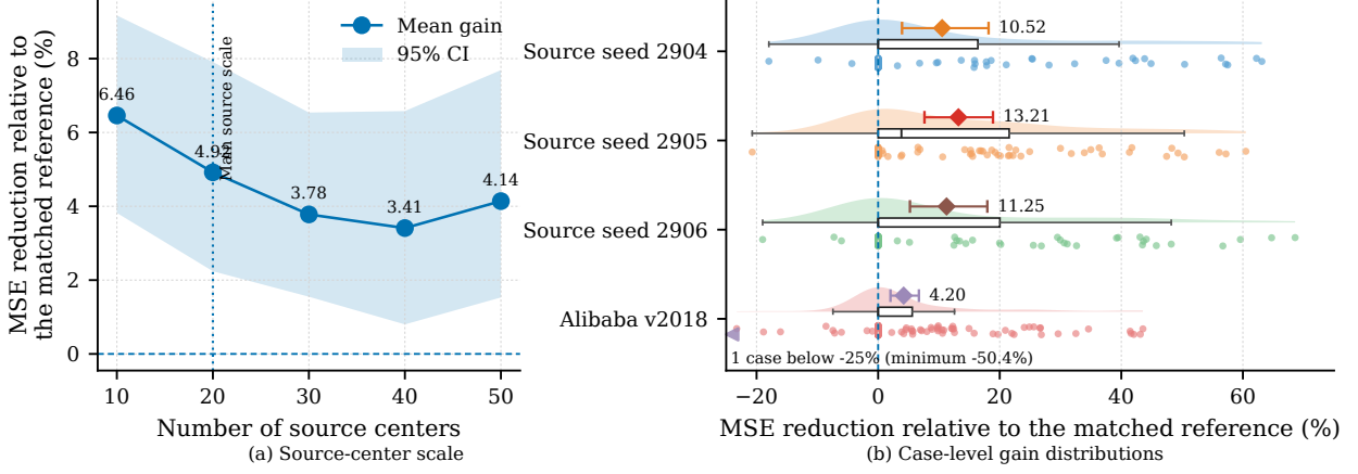
Figure S4: Sensitivity to source conditions and external workload data. (a) Paired MSE reduction relative to the matched reference at each source-center scale; shading shows 95% confidence intervals. (b) Case-level reductions for three source-training seeds and the held-out Alibaba cases under the frozen \tau = 0.10 rule. One Alibaba case below -25\% is clipped only for display; all original values are retained in the analysis.
