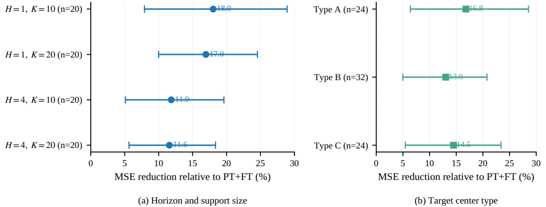
Figure 7: Paired MSE reduction relative to PT+FT across (a) prediction horizons and support sizes and (b) target-center types. Error bars show 95% confidence intervals.
