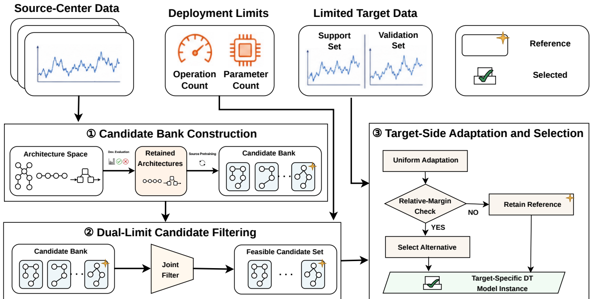
Figure 2: Overall workflow of candidate-bank construction, deployment filtering, and target-side adaptation and selection.
