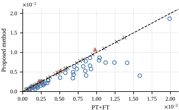
(a) WMSE
