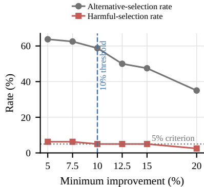
(c) Threshold calibration
