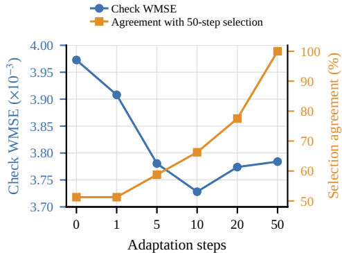
(b) Fixed adaptation budget
