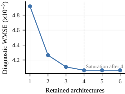
(a) Candidate-bank size
