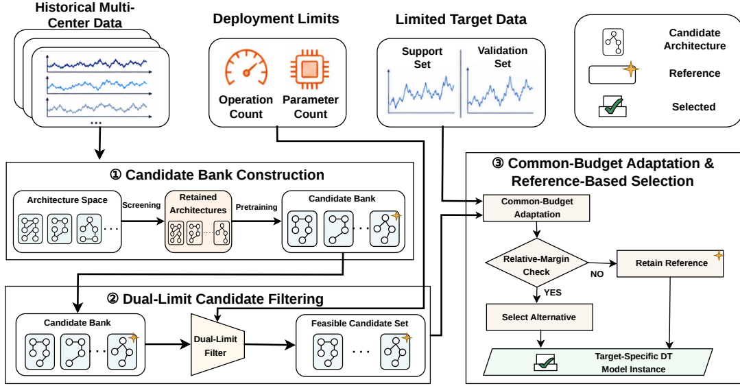
Figure 2: Overall workflow of MSA-DTI: candidate bank construction, dual-limit candidate filtering, and common-budget adaptation with reference-based selection.
