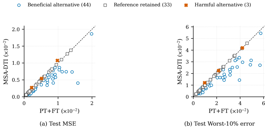
Figure 6: Held-out paired comparison of MSA-DTI and PT+FT for (a) test MSE and (b) test Worst-10% error; beneficial and harmful alternative labels are defined by test MSE, and points below the diagonal favor MSA-DTI.
