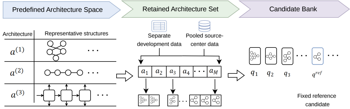
Figure 3: Candidate bank construction and reference candidate selection.
