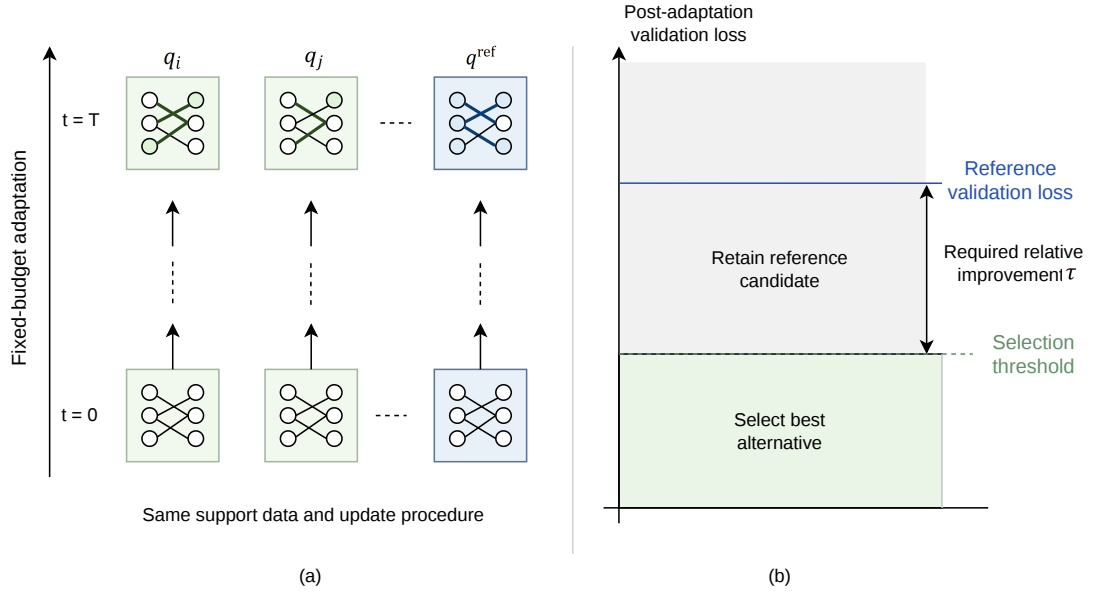
Figure 4: Common-budget adaptation and reference-based selection.
