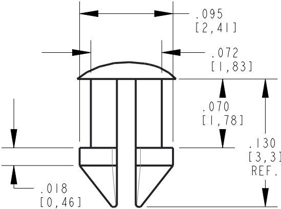
DETAIL A SCALE 10.000
