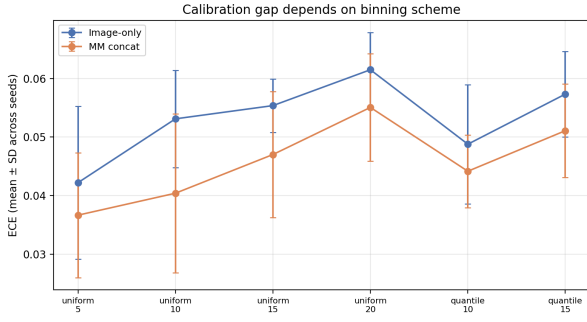
Fig. 9 ECE under different binning schemes; the image–concat calibration gap depends on the binning choice.
