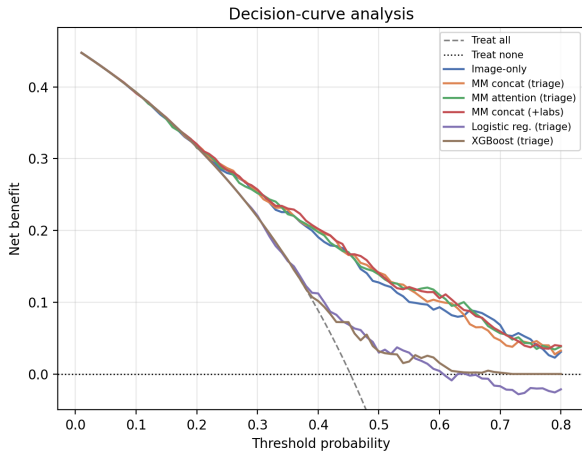
Fig. 8 Decision-curve analysis: net benefit versus threshold probability. Imaging models dominate the triage baselines and reference strategies.
