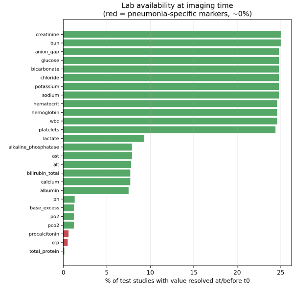
Fig. 7 Fraction of test studies with each laboratory value resolved at or before t_0 ; pneumonia-specific markers (red) are essentially unavailable at imaging time.
