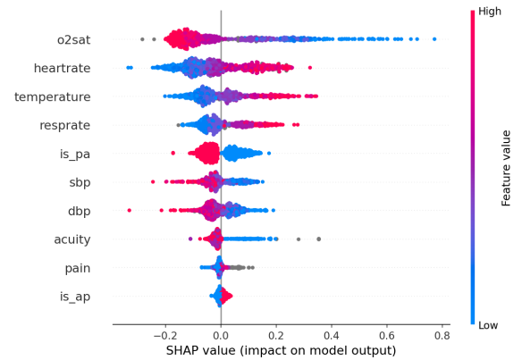
Fig. 10 SHAP summary (beeswarm) for the triage XGBoost model; low SpO 2 pushes predictions toward pneumonia.
