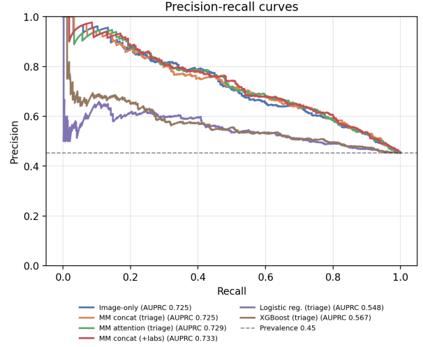
Fig. 2 Precision-recall curves at test prevalence 45.3%.
