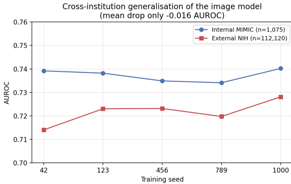
Fig. 12 Cross-institution generalisation: per-seed AUROC on internal MIMIC ( n=1,075 ) versus external NIH ChestX-ray14 ( n=112,120 ); mean drop -0.016 .
