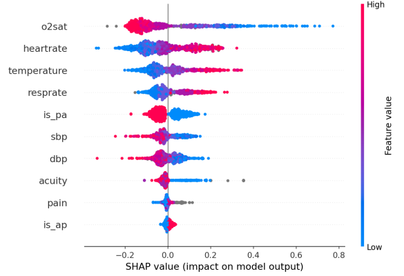
Fig. 12 SHAP summary (beeswarm) for the triage XGBoost model; low SpO 2 pushes predictions toward pneumonia.
