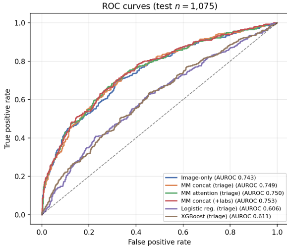
Fig. 1 ROC curves on the held-out test set (5-seed mean predictions for the deep models; AUROC of the ensemble curve shown, slightly above the per-seed means in Table 3).
