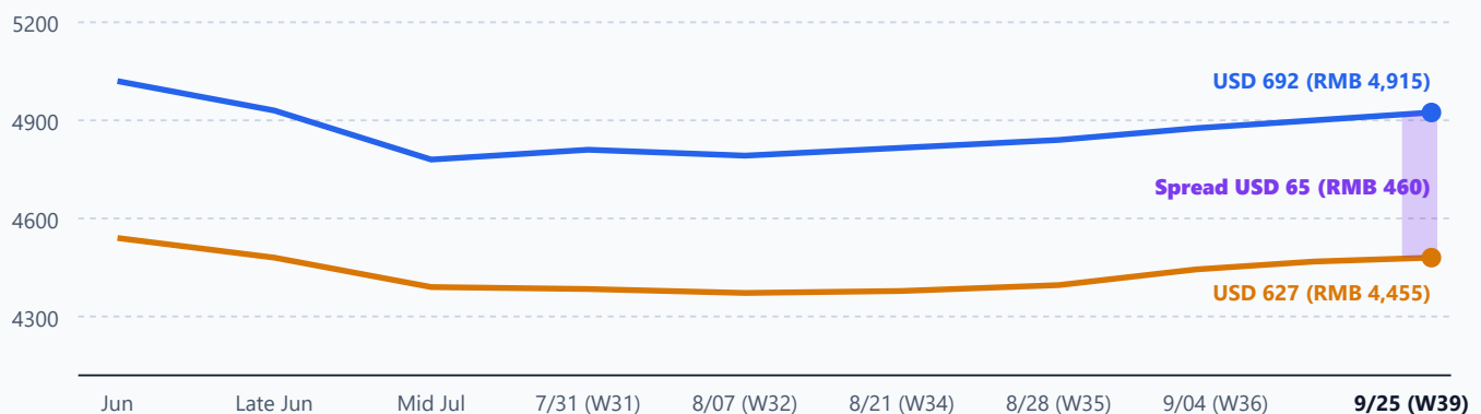
Chart 1 | China NBSK vs. BHKP Spot Pulp Spread Dynamics (2026-06 ~ 2026-09-25)
