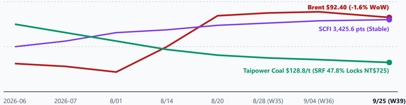
Chart 5 | Global Energy, Maritime SCFI & Taiwan Mill Steam Costs (2026-09-25)
