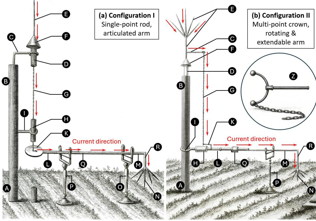
Figura 1. Bertholon’s electrovegetometer, a passive apparatus intended to channel “atmospheric electricity” toward crops. (a) Configuration I, featuring a single-point rod collector (E) at the mast head and an articulated arm that distributed charge through a multi-point crown (N). (b) Configuration II, equipped with a multi-point crown collector (E), a rotating and extendable arm and a larger treatment footprint terminating by a multi-point crown distributor (N). A neutralization device (Z), shown in the inset of (b), could provide safety and on/off control. Adapted from [Bertholon, 1783].
