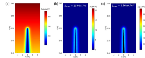
Figure 3. Pre-corona response of the upper single-point rod collector (apex angle \theta = 4^\circ ) under fair-weather forcing ( j_0 \approx 2 \text{ nA/m}^2 , E_0 \approx 2 \text{ kV/m} , V_0 \approx 300 \text{ V} ).
