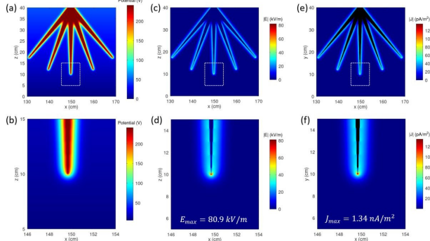
Figure 4. Pre-corona response of the lower five-point crown under fair-weather forcing ( E_0 \approx 3 kV/m, \rho \approx 10^{-14} C/m³) with apex angle \theta
