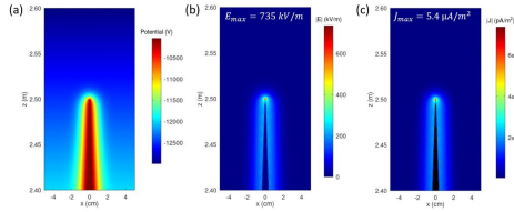
Figura 5. Response of the single-point rod collector under idealized storm-like forcing ( \approx . , \approx . ). (a) Steady potential V showing deep compression of equipotentials near the floating metal apex. (b) Electric-field magnitude || reaching = . , approaching empirical corona-onset ranges. (c) Current-density magnitude || peaking at = . \mu\text{A/m}^2 . Values represent límites superiores pre-corona within the linear, space-
