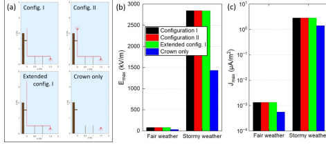
Figura 8. (a) Four distinct geometries of the electrovegetometer used in the simulations. Brown regions denote wooden supports, red lines metallic conductors. (b) Maximum electric field at the lower crown distributor, E_{max} , under fair-weather and storm-like forcing, showing that all mast-bearing configurations produce similar peak fields while the crown-only case remains lower in the storm regime. (c) Corresponding maximum conduction current density, J_{max} , on a logarithmic scale, illustrating the three-order-of-magnitude increase from fair to storm conditions and the enhanced currents obtained when an elevated metallic mast is present.
