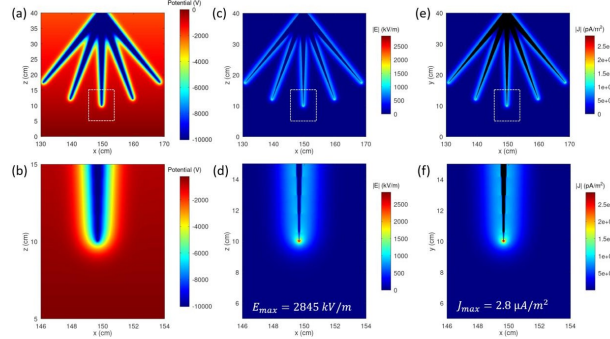
Figura 6. Response of the lower five-point crown under idealized storm-like forcing ( \approx . , \approx . ). (a,b) Potential V showing a deeply collapsed well and strong confinement of equipotentials around each apex. (c,d) Electric-field magnitude || with a localized maximum = . . , approaching empirical breakdown ranges. (e,f) Current-density magnitude || peaking at = . \mu\text{A/m}^2 . These values represent upper-bound, pre-discharge fields within the linear, space-charge-free model.
