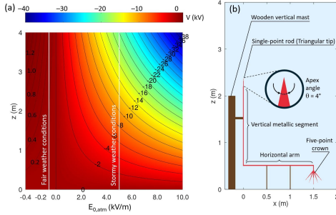
Figura 2. (a) Electric potential ( V ) in the atmosphere above the ground, shown as colored contours (in kV) and black iso-potential lines. The horizontal axis represents the imposed vertical electric field E_{0,atm} , ranging from fair-weather values ( E_{0,atm} < 0 ) to storm-time values ( E_{0,atm} > 0 ). The two white vertical lines correspond to the fair-weather and stormy-weather atmospheric conditions for this study. (b) Geometrical model of Bertholon's electrovegetometer as implemented in configuration I, which includes
