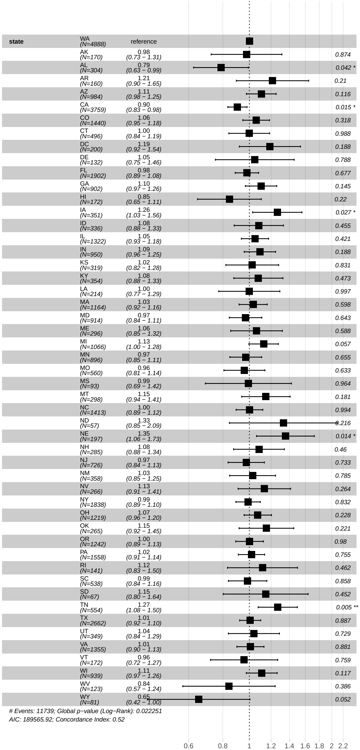
Unadjusted Hazard Ratio
